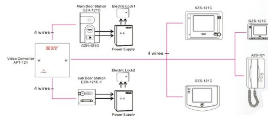
Two Door Stations and Four Door Phones
